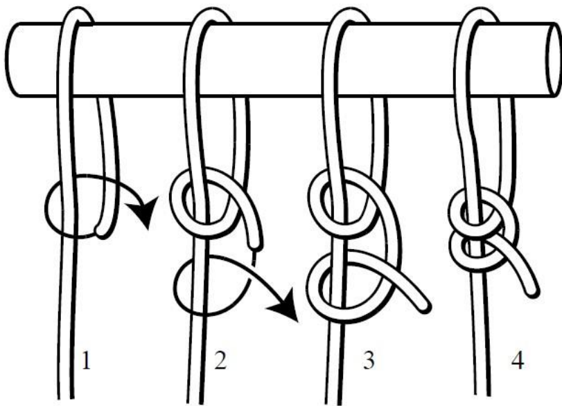
TwoHalf-Hitches
